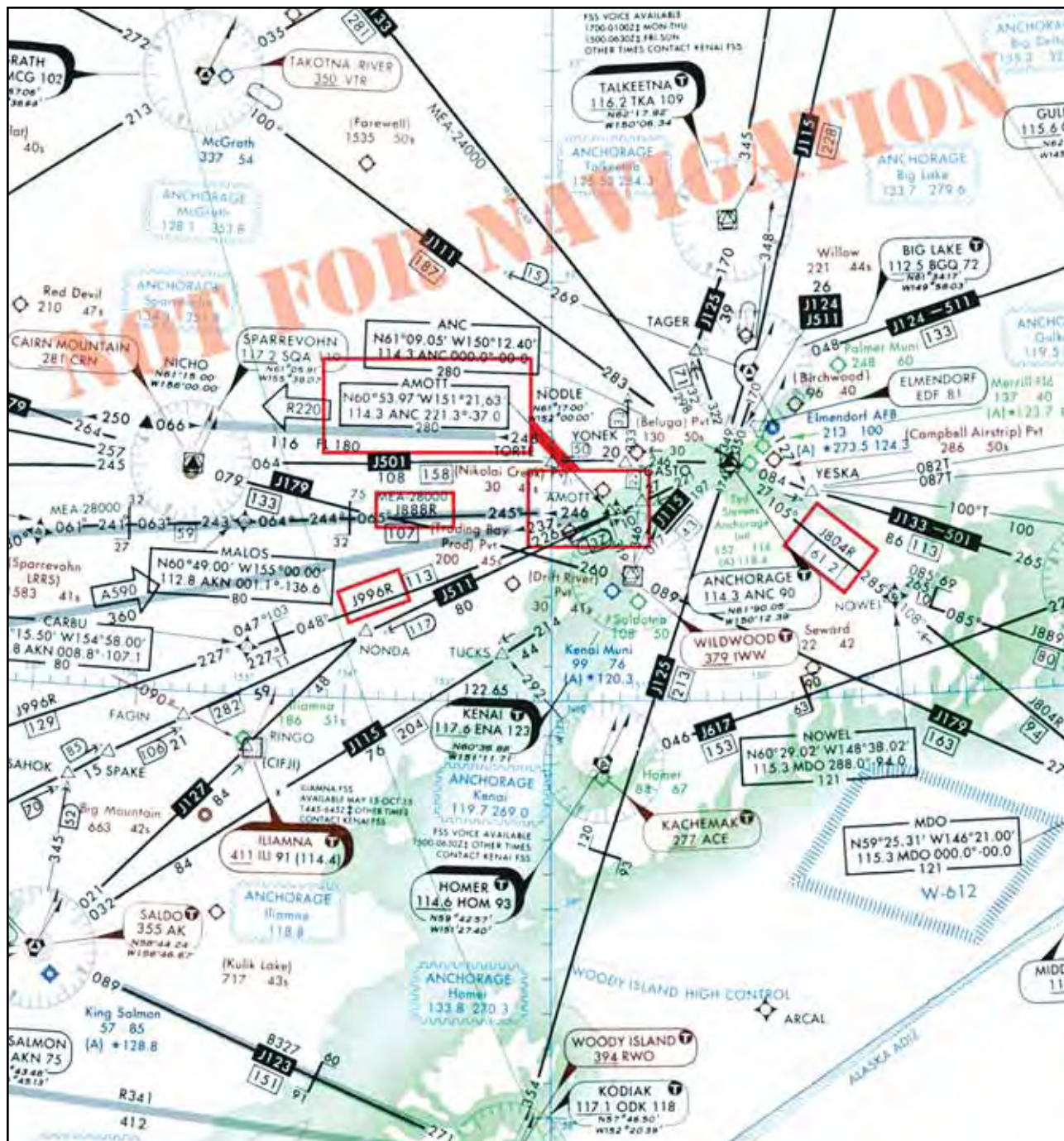
Figure 3-37. Published RNAV Jet Routes.
