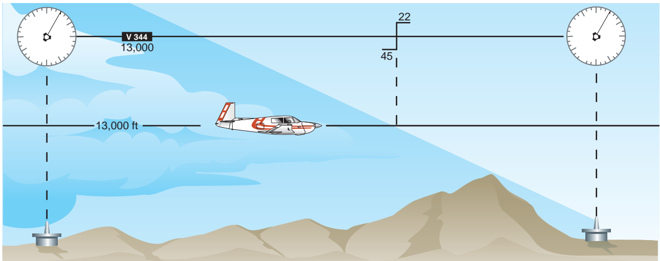
Figure 3-15. Changeover Points.
