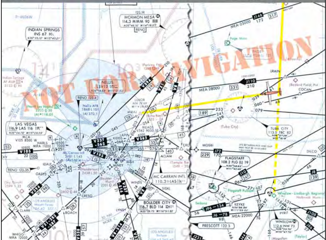
Figure 3-35. Random RNAV Route.
