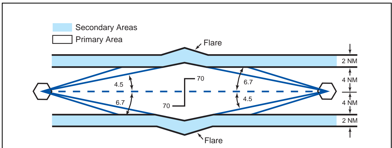
Figure 3-16. Changeover Point Effect on Long Airways or Route Segment.
